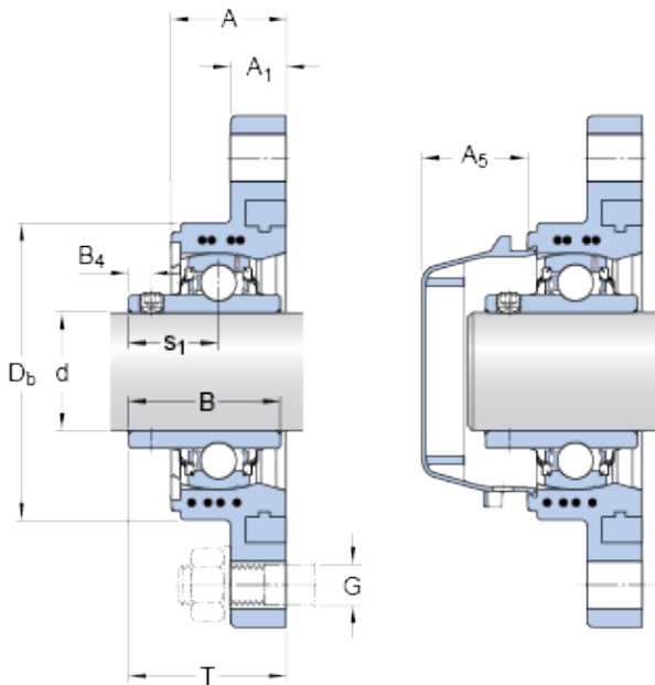
FYTWK 1.3/16 YTH Bearing 2D drawings and 3D CAD models
